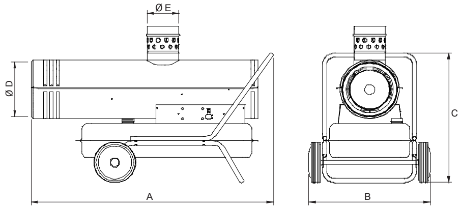
GRY – I Indirect heater with wheels.
