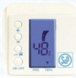
LCD screen with R.H. % indicator and electronic humidistat
