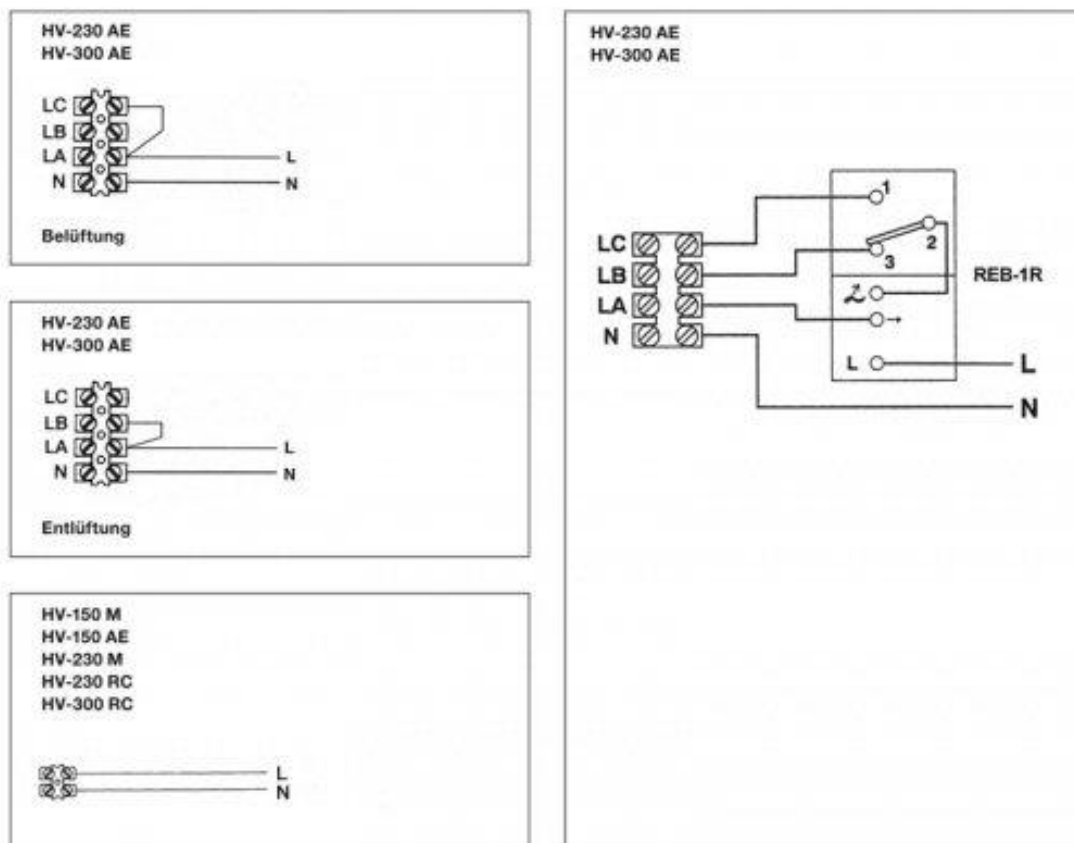
HV-STYLVENT electrical scheme
