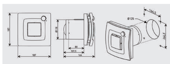
DIMENSIONS (mm)
