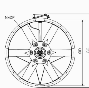
TGT 1400 and TGT 1600 Short casing
