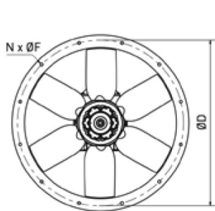
TGT ATEX-500 to TGT ATEX-1250 Short casing
