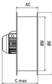
TGT ATEX-400 to TGT ATEX-1250 long casing (LP)
