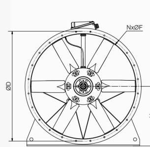
TGT 1400 and TGT 1600 long casing (LP)
