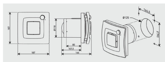
SILENT DUAL-200
