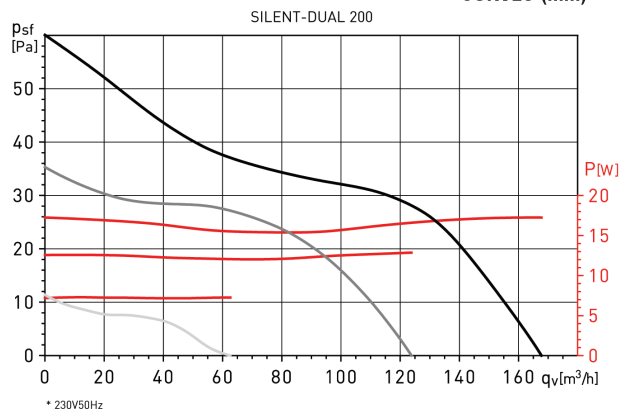
CURVES (mm)
