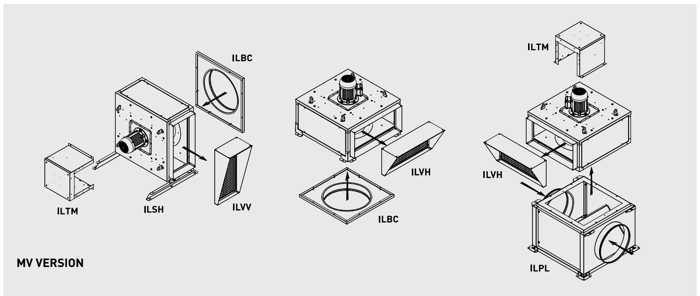
ILSH Mounting support with motor in horizontal position
