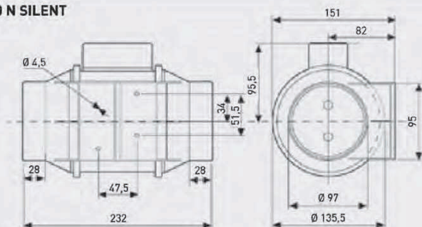
TD-SILENT 250 to 1000
